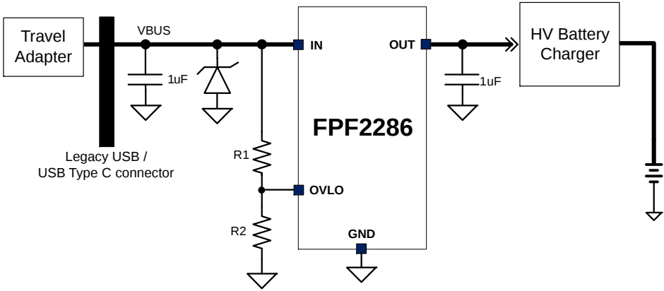
Figure 1. Application Schematic – Adjustable Option
