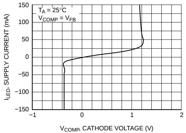
Figure 10b. LED Current vs. Cathode Voltage
