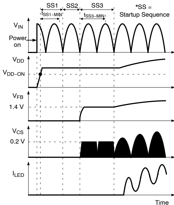
Figure 16. Startup Sequence
