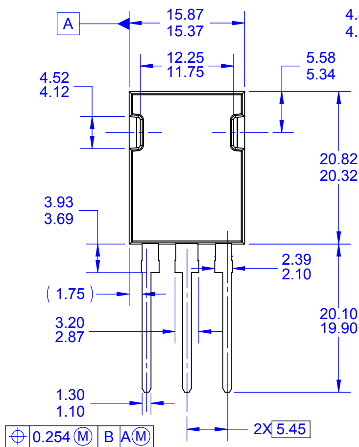
FRONT VIEW
