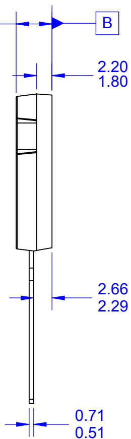
SIDE VIEW
