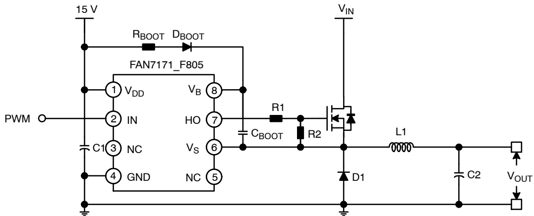
Figure 1. Typical Application
