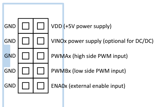
Figure 7. DRIVING (P1 and P3) Connector PINout
