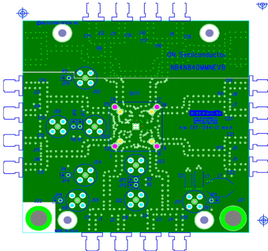
Figure 8. Power Layer
