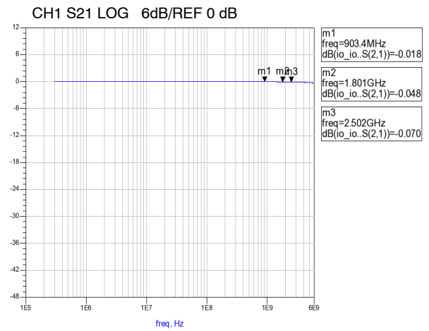
Figure 4. Insertion Loss S21 - I/O to I/O
