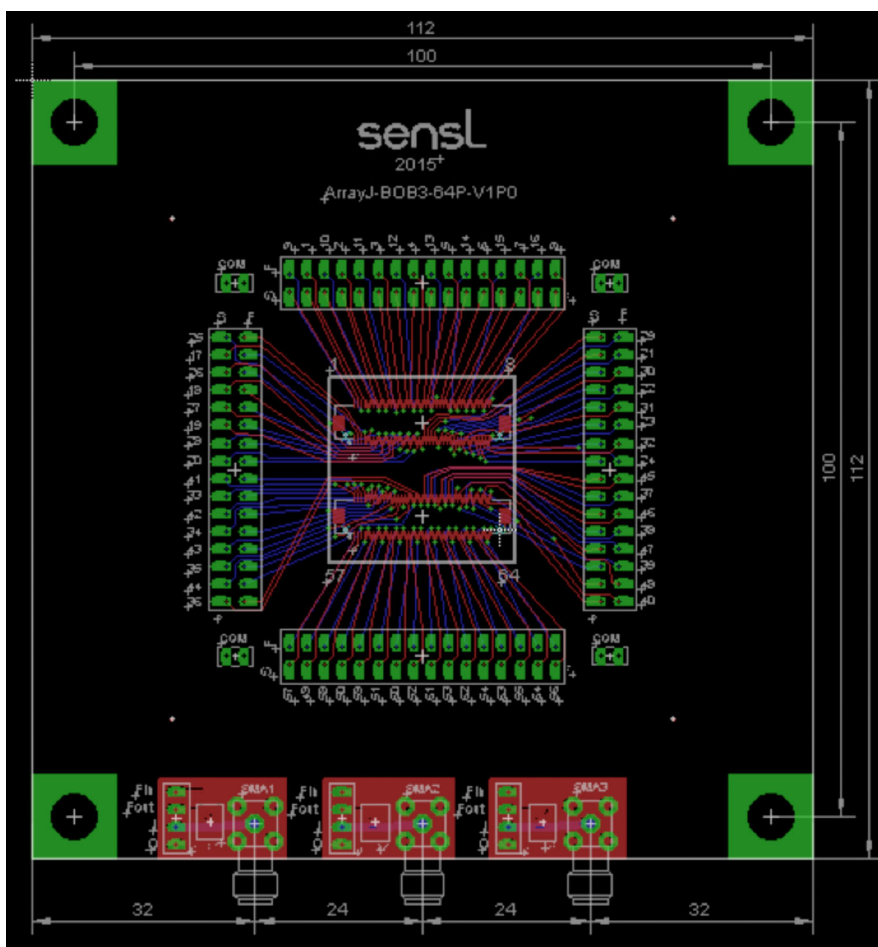
Figure 13. Layout of the ARRAYJ-BOB3-64P. Note that the array corner pixel numbers are shown on the silkscreen of the PCB to ensure correct orientation of the array.
