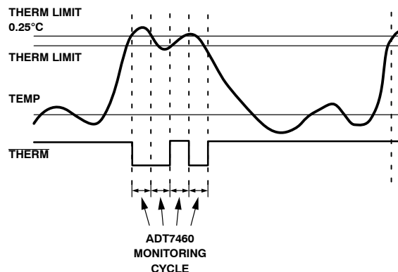
Figure 39. Asserting THERM as an Output, Based on Tripping THERM Limits
