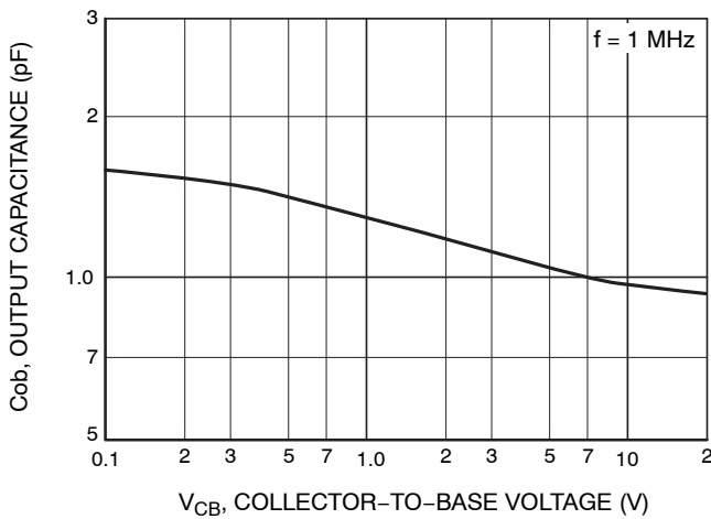
Figure 5. C_{ob} - V_{CB}
