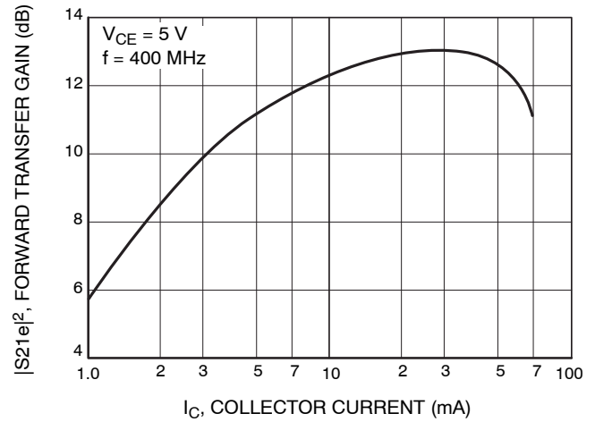
Figure 8. |S_{21e}|^2 – I_C
