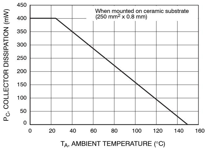
Figure 9. P_C – T_A
