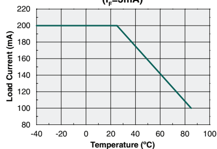
Maximum Load Current vs. Temperature ( I_F=3\text{mA} )
