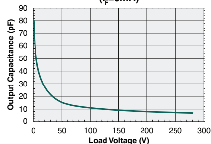
Output Capacitance vs. Load Voltage ( I_F=0\text{mA} )
