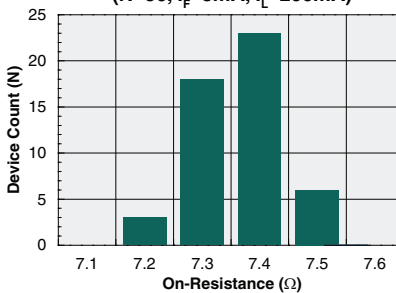
Typical On-Resistance Distribution (N=50, I_F=3\text{mA} , I_L=200\text{mA} )
