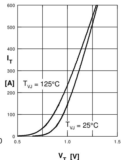
Fig. 9 Forward characteristics
