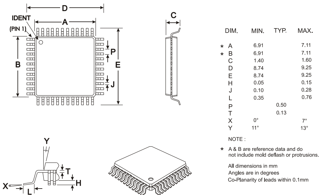
Figure 27 Mechanical Outline of 48-pin LQFP (L4)
