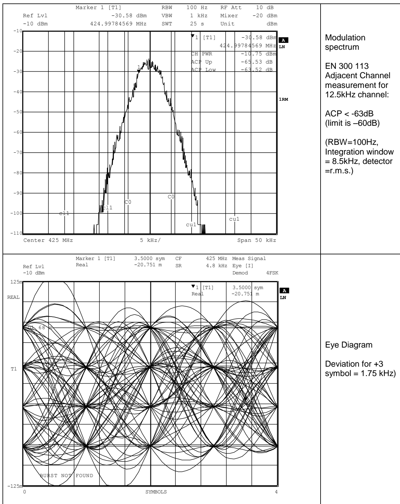
Figure 20 Tx Modulation Spectra (4FSK), 9600bps (4800 symb/s), 2point modulation
