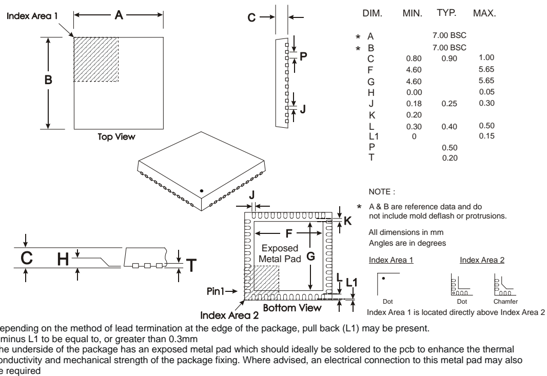
Figure 26 Mechanical Outline of 48-pin VQFN (Q3)
