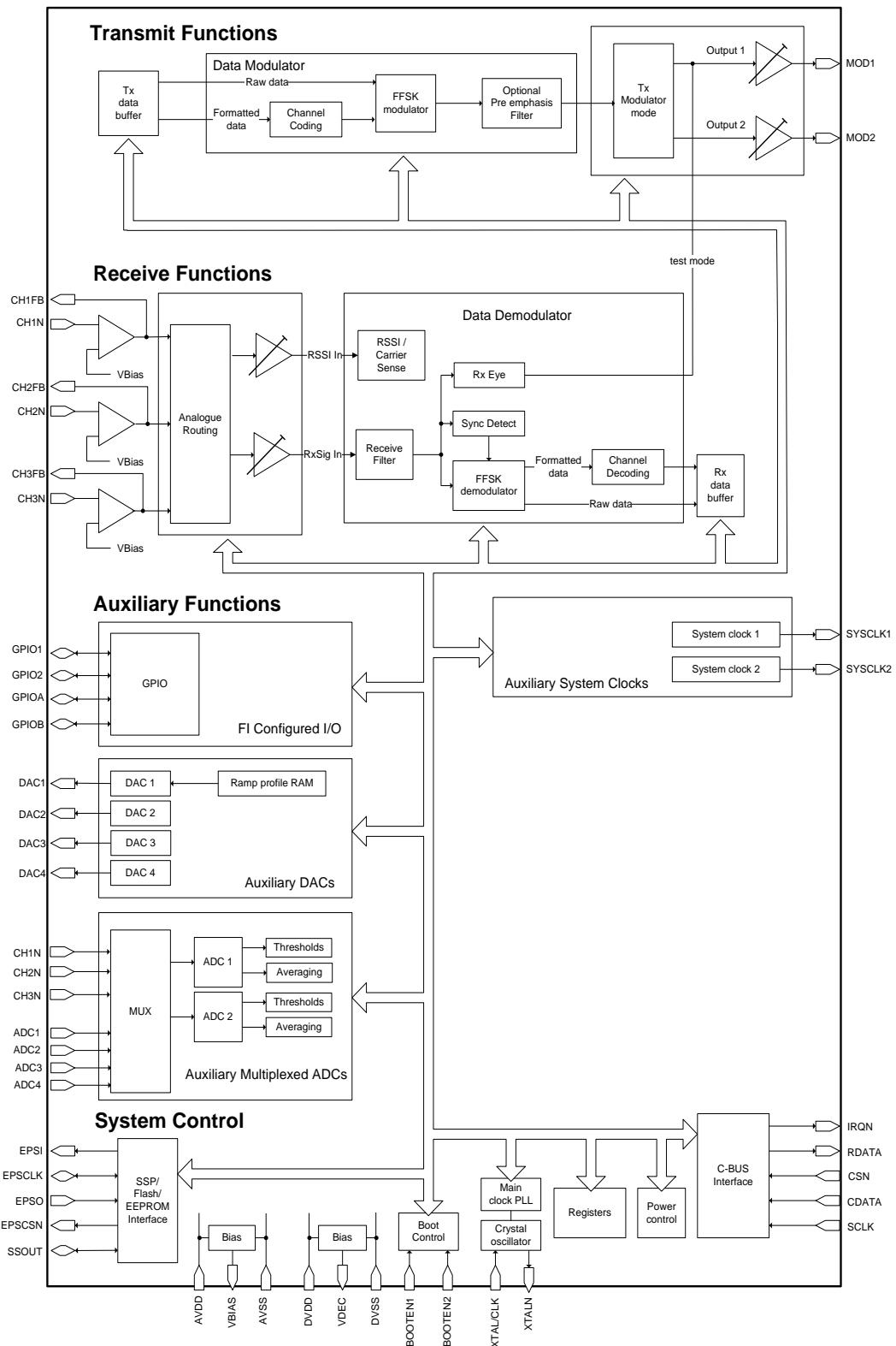
Figure 1 Block Diagram
