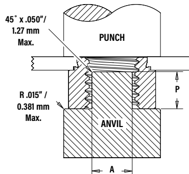
PROTRUSION ANVIL Thread Sizes 3/8 and M10
