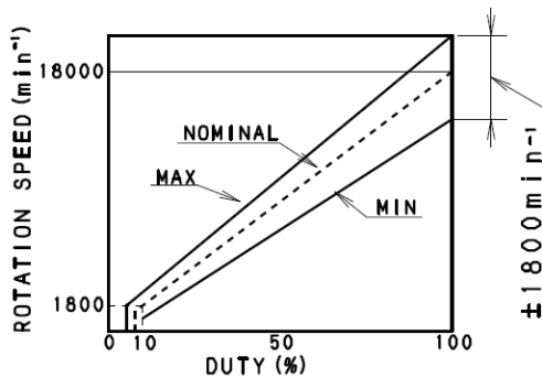
Detail of PWM curve(At 0~100%)
