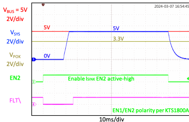
Active-High Enable/Soft-Start in ISINK Mode ( V_{BUS} = 5V , EN1 = 0 , R_{LOAD\_V_{SYS}} = 100\Omega , R_{LOAD\_POK} = 300\Omega )
