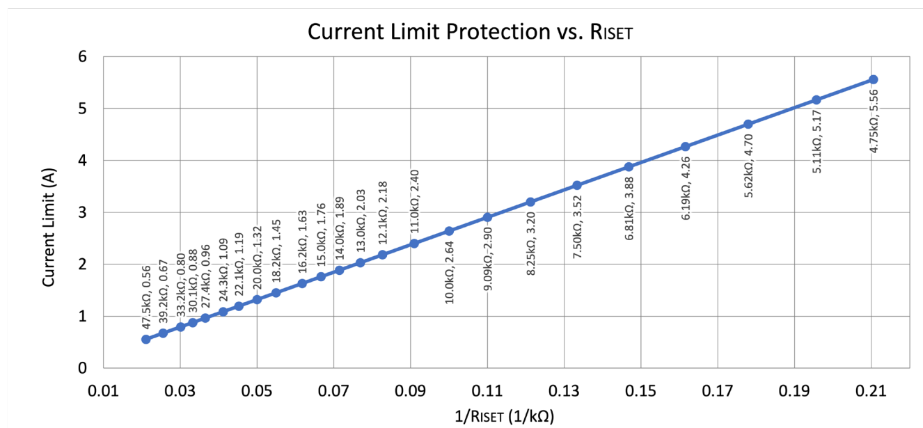
Figure 4. ISOURCE Mode Current Limit Protection vs. RSET Resistance
