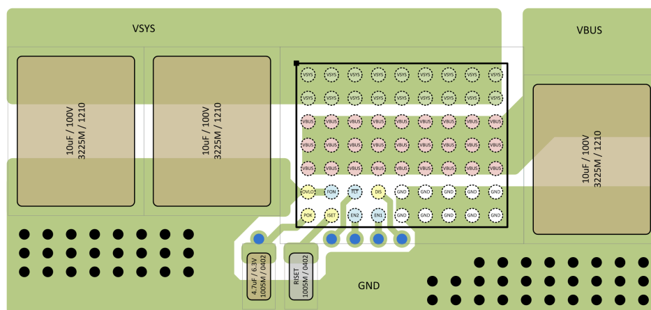
Figure 5. Recommended PCB Layout
