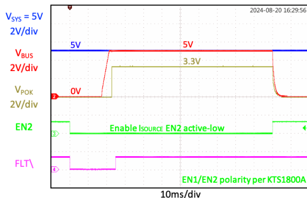
Active-Low Enable/Soft-Start in ISOURCE Mode ( V_{SYS} = 5V , EN1 = 1 , R_{LOAD\_VBUS} = 100\Omega , R_{LOAD\_POK} = 300\Omega )
