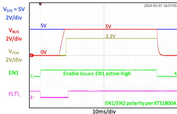
Active-High Enable/Soft-Start in ISOURCE Mode ( V_{SYS} = 5V , EN2 = 0 , R_{LOAD\_VBUS} = 100\Omega , R_{LOAD\_POK} = 300\Omega )
