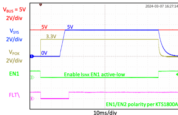
Active-Low Enable/Soft-Start in ISINK Mode ( V_{BUS} = 5V , EN2 = 1 , R_{LOAD\_V_{SYS}} = 100\Omega , R_{LOAD\_POK} = 300\Omega )
