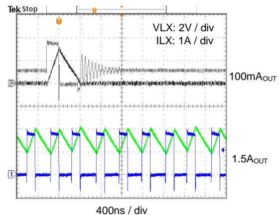
V_{LX} and I_{LX} Switching Waveforms (V_{OUT} = 1.15625V, \text{Mode} = \text{Auto})
