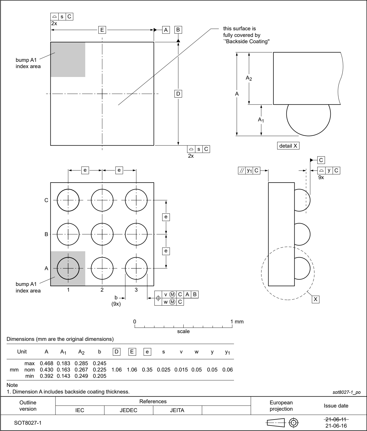
Fig. 12. Package outline SOT8027-1 (WLCSP16)
