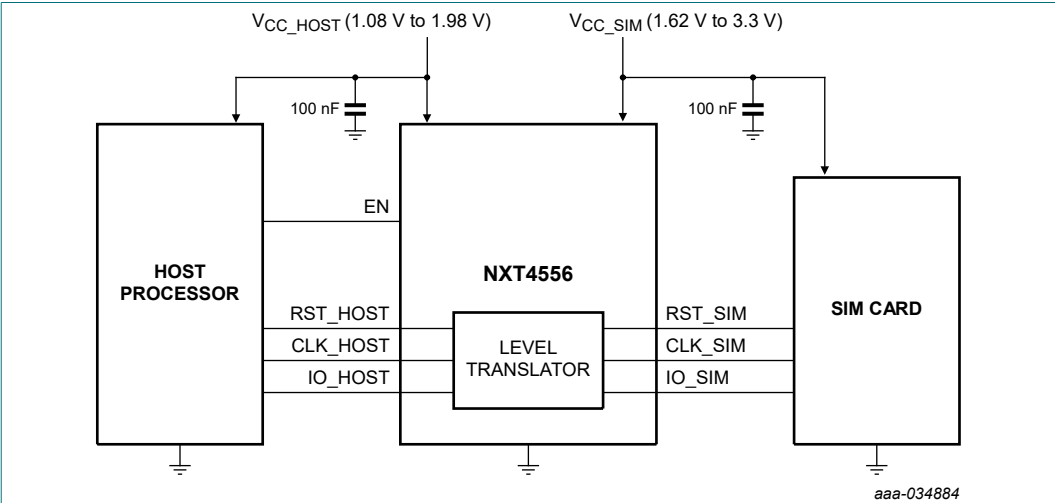
Fig. 10. NXT4556 application circuit interfacing with typical SIM card
