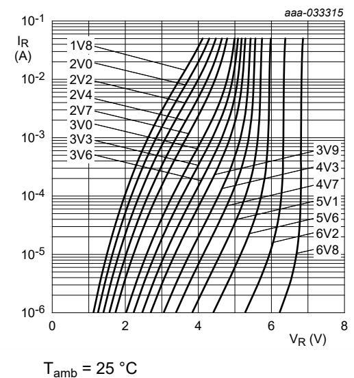
Fig. 5. Reverse current as a function of reverse voltage; typical values (BZX8450-B/C1V8-Q to BZX8450-B/C6V8-Q)
