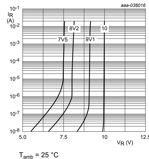
Fig. 6. Reverse current as a function of reverse voltage; typical values (BZX8450-B/C7V5-Q to BZX8450-B/C10-Q)
