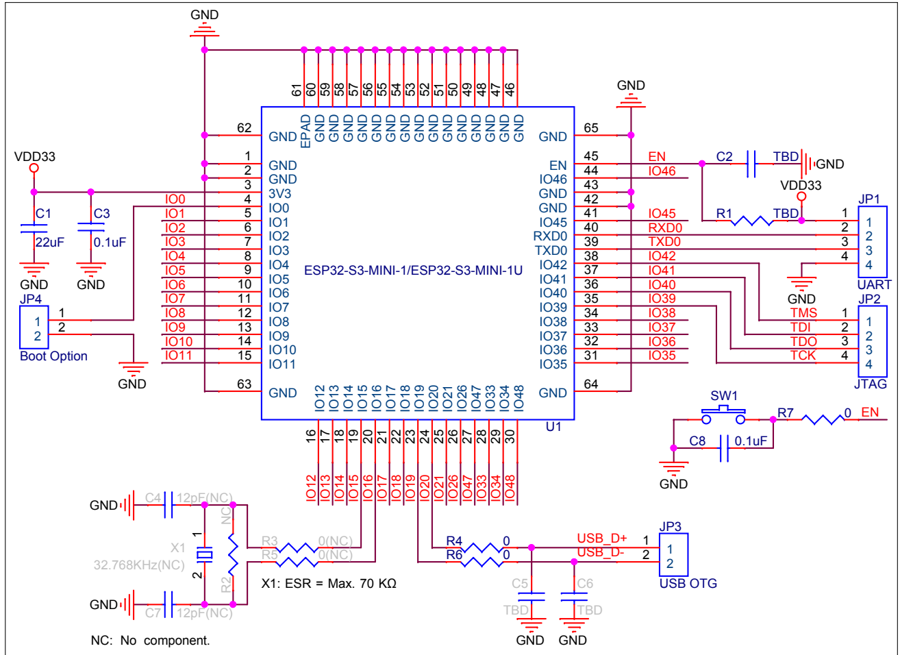
Figure 9-1. Peripheral Schematics
