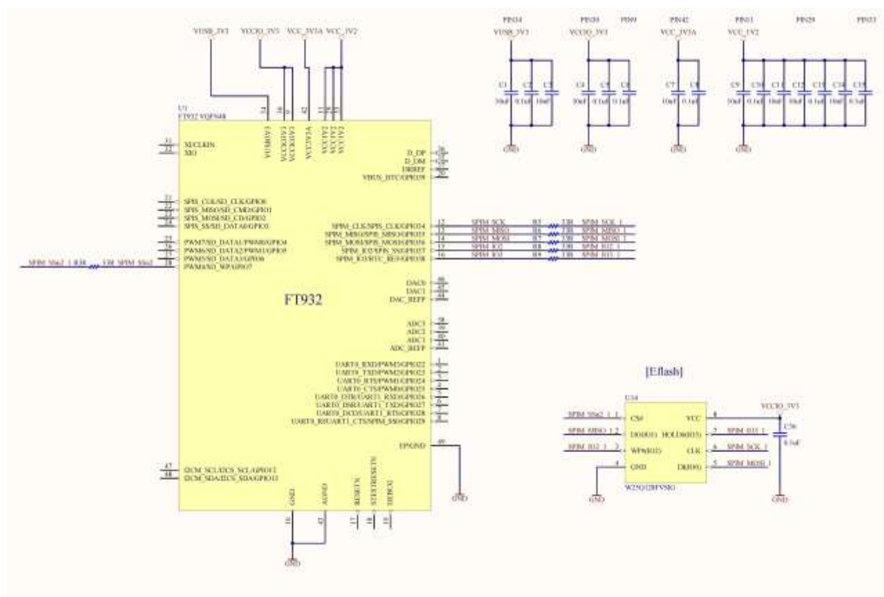
Figure 4-5 – Flash Memory Interface
