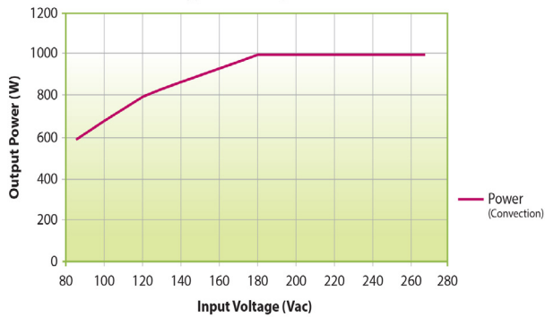
CX10 Input Voltage Typical Derating Curve
