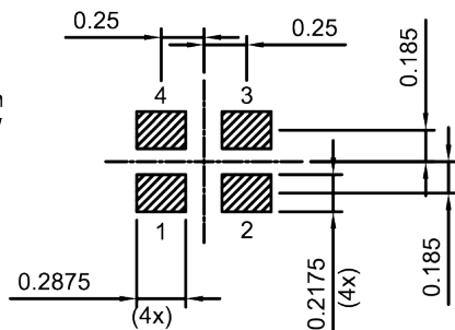
Figure 2: Drawing of package with package height A = 0.56 mm (max.). See Sec. Package information (p. 18).
