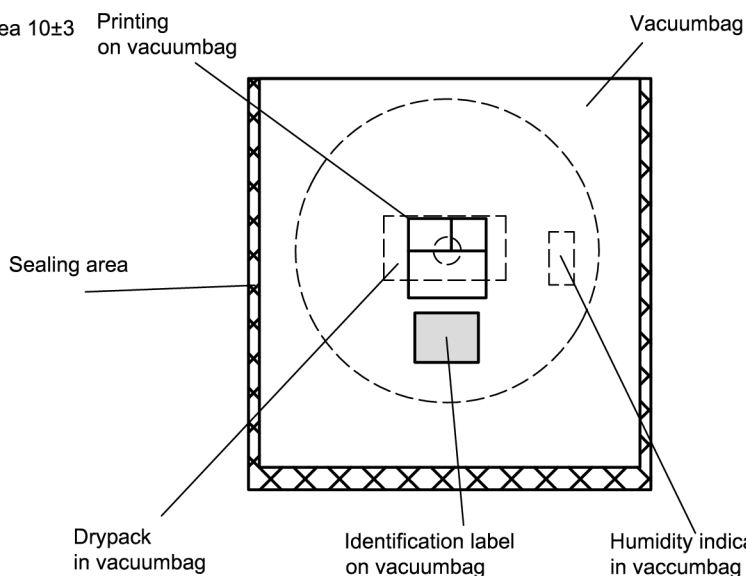
Figure 9: Drawing of moisture barrier bag (MBB) for reel with diameter of 180 mm.
