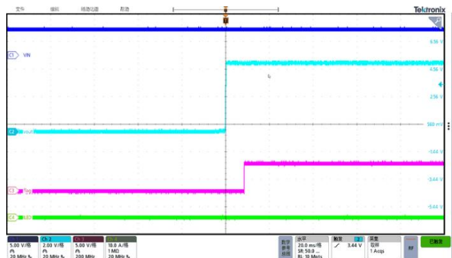
Figure 13. Short to no load transient response
