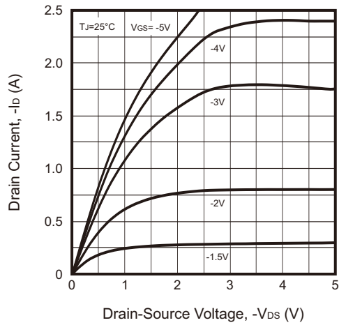
Fig.1 - Output Characteristics
