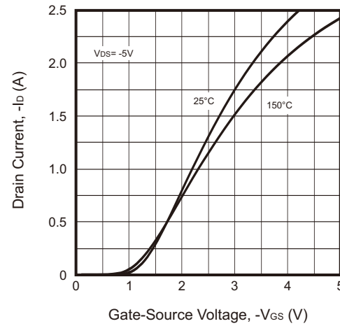
Fig.2 - Transfer Characteristics
