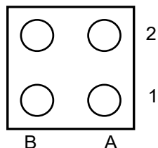
RP122Z (WLCSP-4-P8 / WLCSP-4-P12) Pin Configuration
