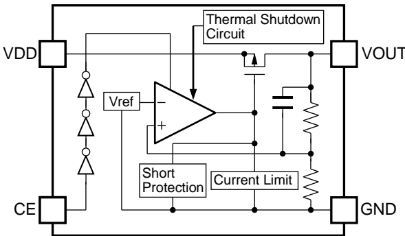
R1560x Block Diagram
