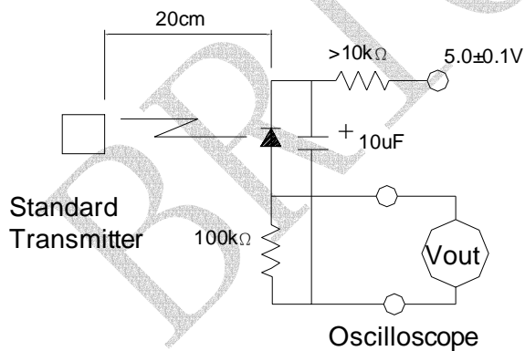
Fig.2 Measuring Method
