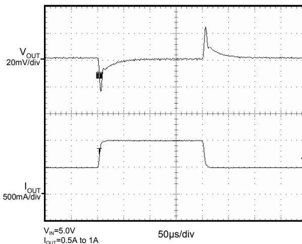
Transient Response ( V_{OUT}=1.0V )
