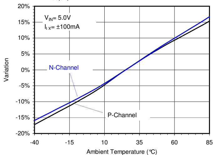
R_{DS(ON)} Variation vs. Temperature
