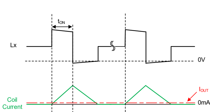
XCL242 series: Example of light load operation
