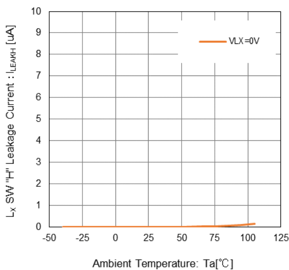
(10) Lx SW "H" Leakage Current vs. Ambient Temperature
