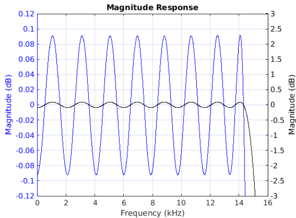
Figure 7-1. Passband Magnitude
