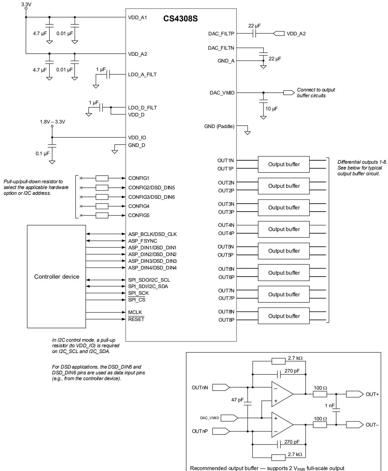
Figure 2-1. Typical Connections
