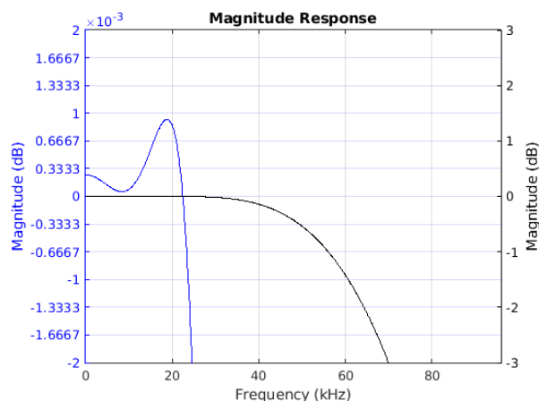
Figure 7-43. Passband Magnitude
