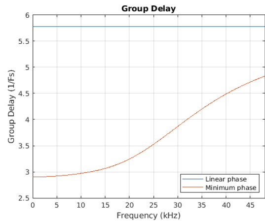
Figure 7-30. Group Delay vs. Frequency
