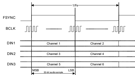
Figure 4-18. Left-Justified Data Format
