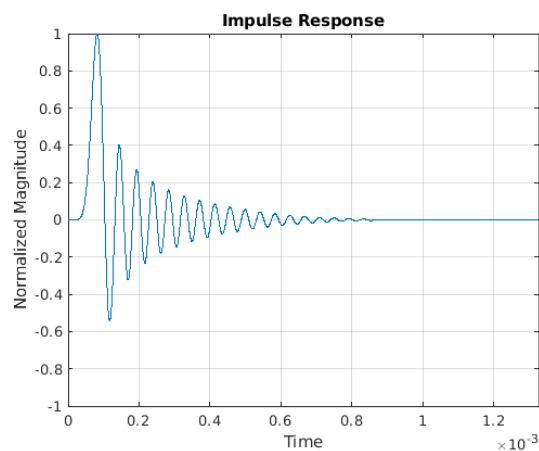
Figure 7-10. Impulse Response—Minimum Phase
