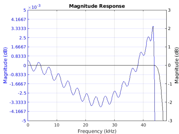
Figure 7-19. Passband Magnitude
