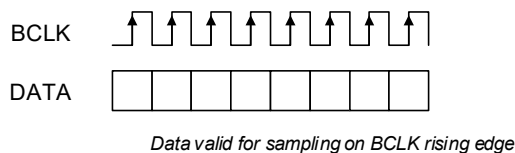
Figure 4-10. Noninverted BCLK
