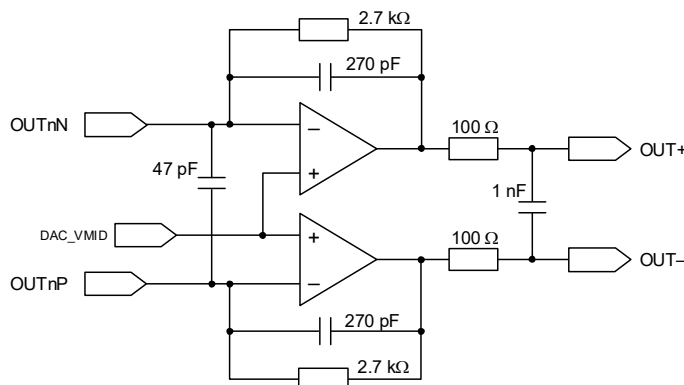
Figure 4-3. Output Buffer
