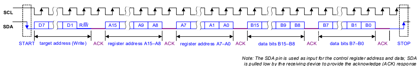
Figure 4-30. Control Interface I 2 C Register Write
