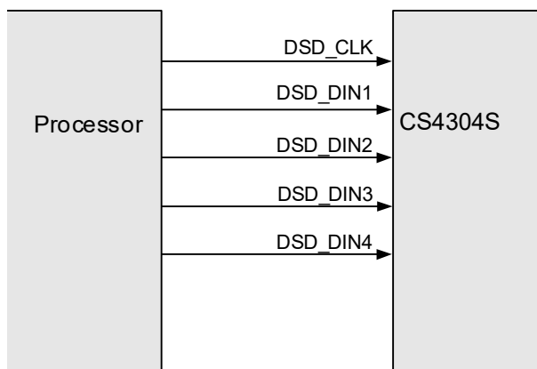
Figure 4-26. DSD Interface Connection
