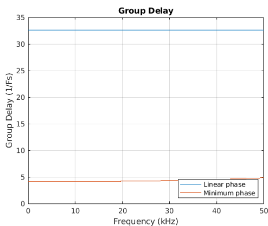
Figure 7-42. Group Delay vs. Frequency
