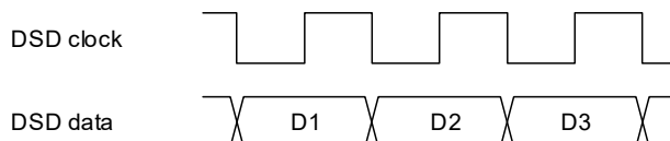
Figure 4-27. DSD Interface Timing
