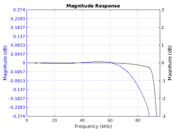
Figure 7-37. Passband Magnitude
