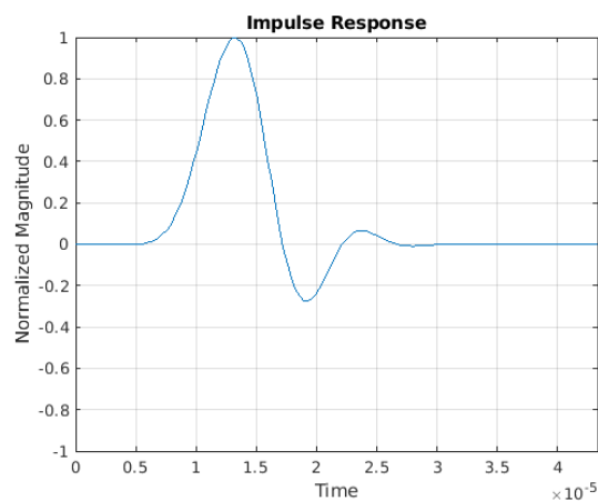
Figure 7-76. Impulse Response—Minimum Phase
