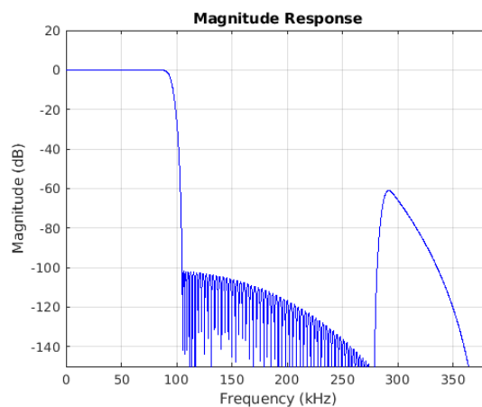
Figure 7-38. Stopband Magnitude
