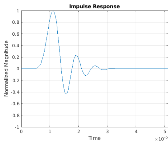
Figure 7-70. Impulse Response—Minimum Phase
