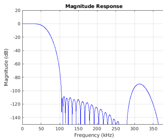
Figure 7-50. Stopband Magnitude
