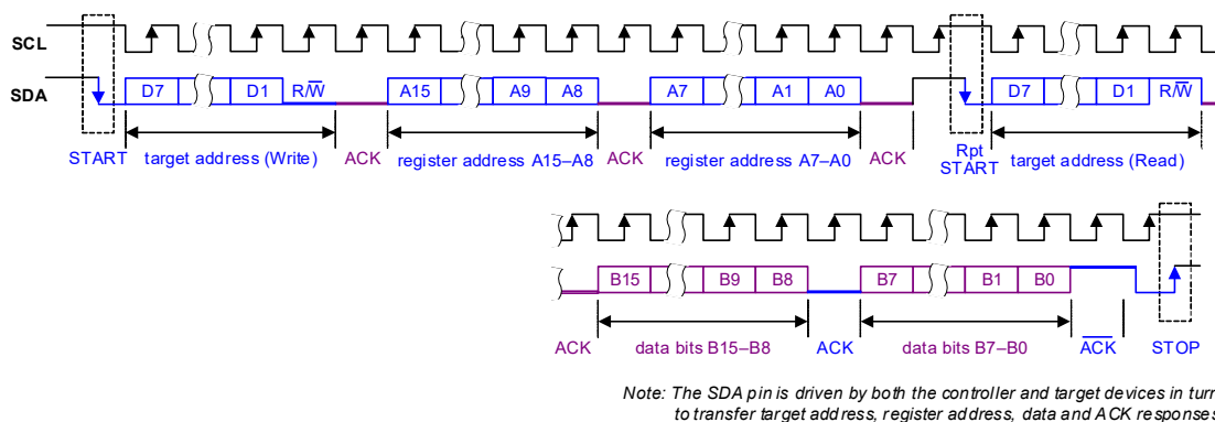
Figure 4-31. Control Interface I 2 C Register Read
