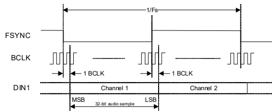
Figure 4-17. I2S Data Format
