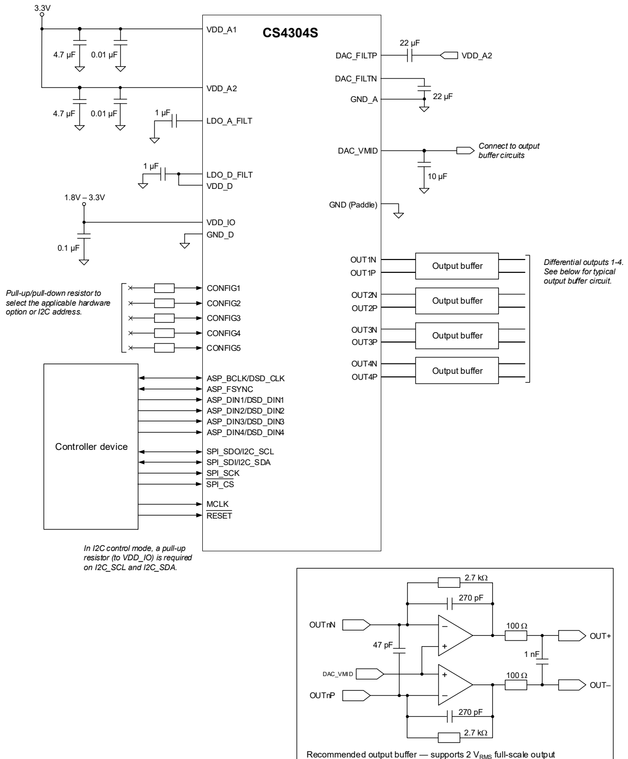
Figure 2-1. Typical Connections
