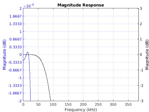
Figure 7-73. Passband Magnitude
