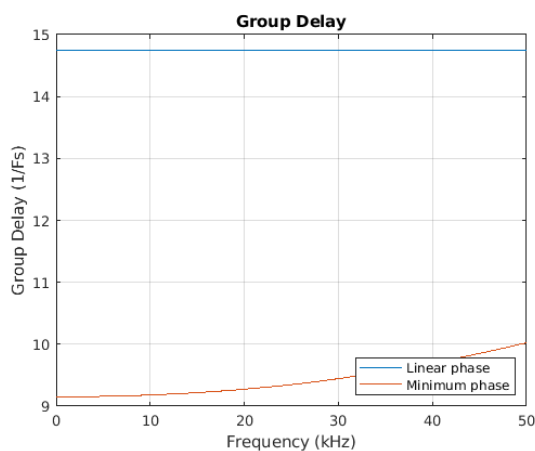
Figure 7-78. Group Delay vs. Frequency
