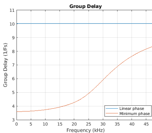
Figure 7-36. Group Delay vs. Frequency
