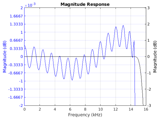
Figure 7-1. Passband Magnitude
