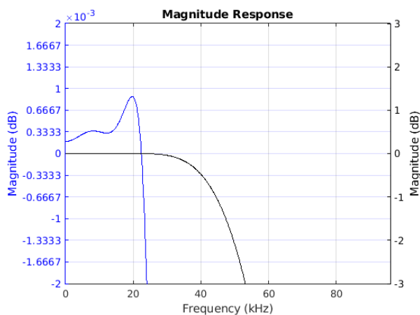
Figure 7-49. Passband Magnitude
