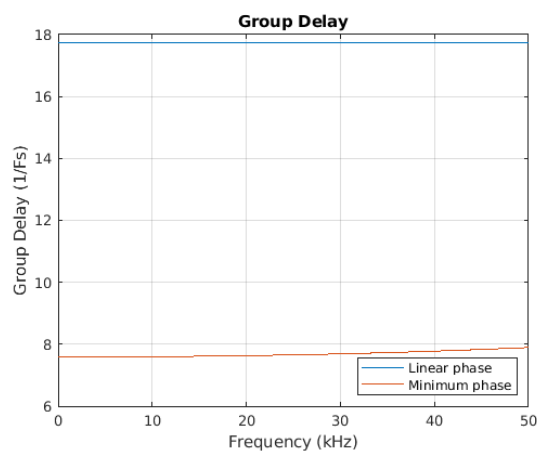
Figure 7-72. Group Delay vs. Frequency
