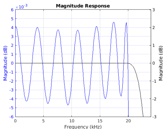
Figure 7-13. Passband Magnitude
