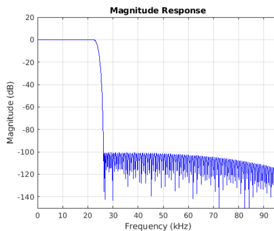
Figure 7-8. Stopband Magnitude
