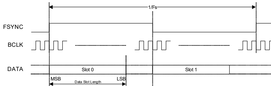
Figure 4-8. Left-Justified Data Format
