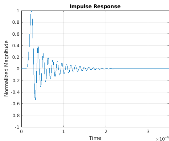
Figure 7-40. Impulse Response—Minimum Phase
