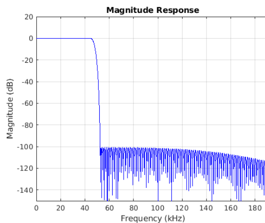
Figure 7-20. Stopband Magnitude
