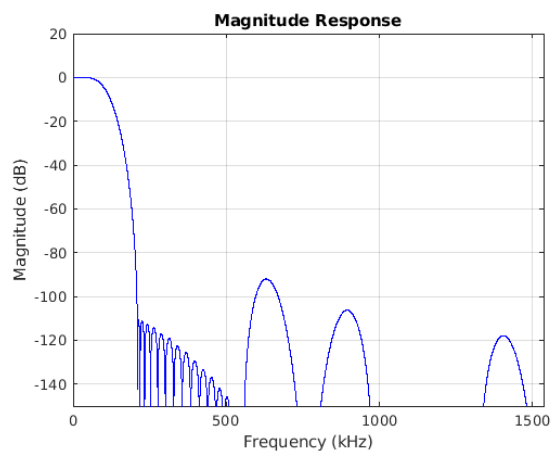
Figure 7-74. Stopband Magnitude
