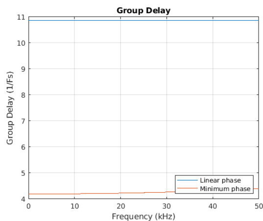
Figure 7-60. Group Delay vs. Frequency
