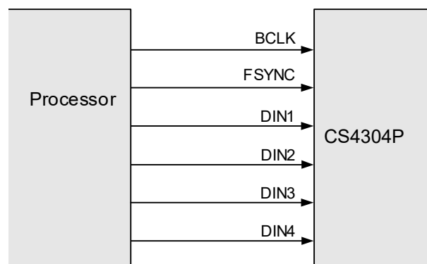
Figure 4-6. Secondary Mode
