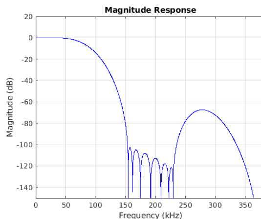
Figure 7-44. Stopband Magnitude
