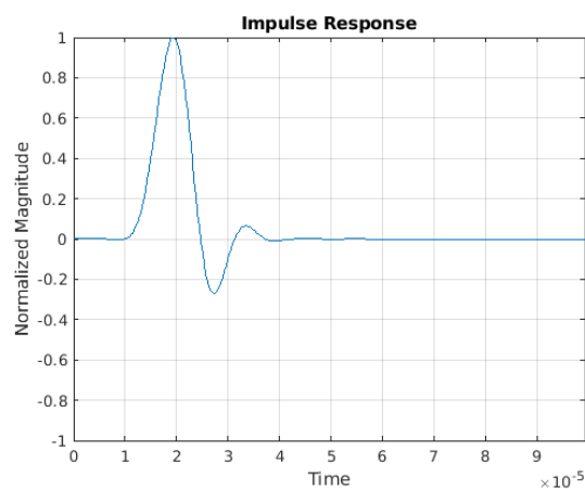
Figure 7-46. Impulse Response—Minimum Phase
