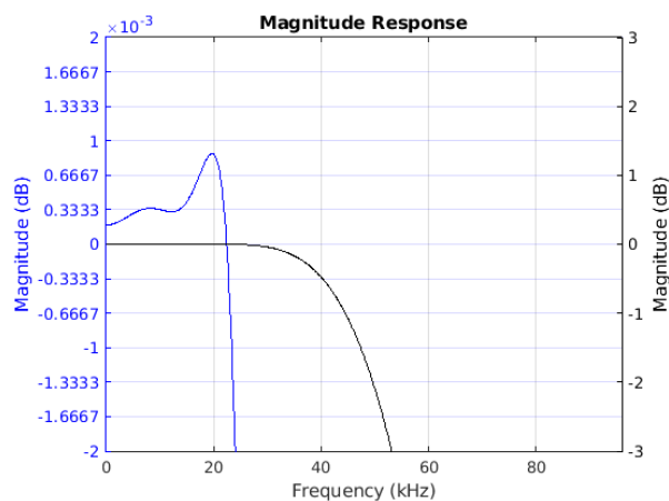
Figure 7-49. Passband Magnitude
