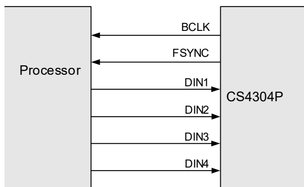
Figure 4-5. Primary Mode
