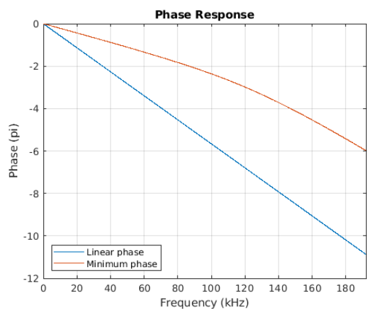
Figure 7-59. Phase vs. Frequency
