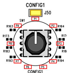
Figure 15: Rotary Switch
