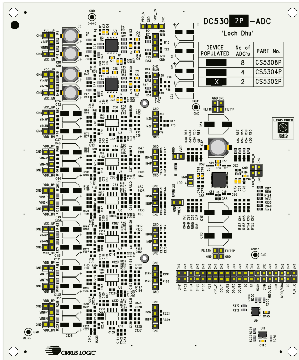
Figure 1: DC5302P-ADC Daughter Card
