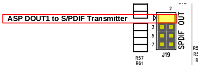
Figure 15: SPDIF IN and SPDIF out Jumper Link Configuration
