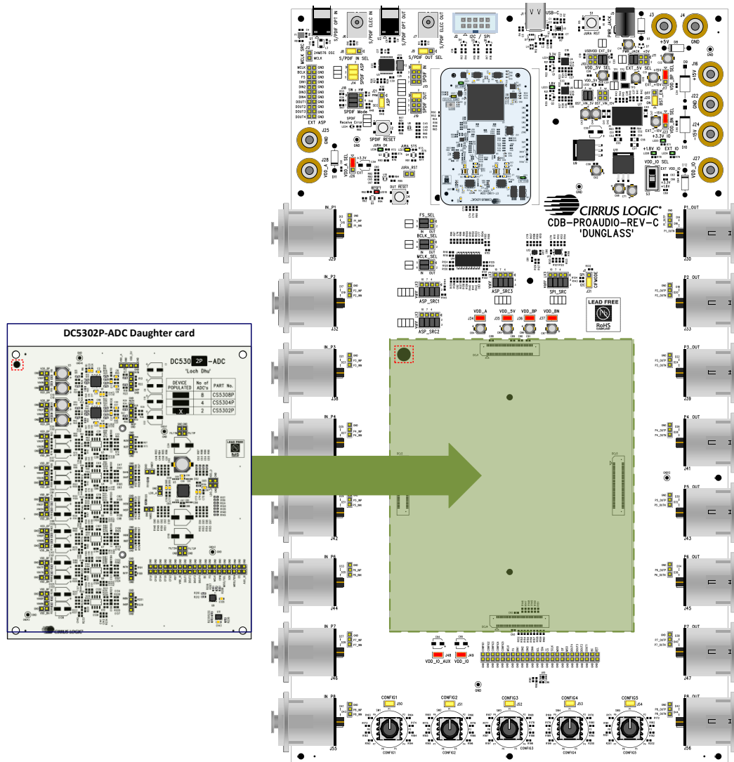
Figure 2: How to Connect DC5302P-ADC onto the Dunglass System
