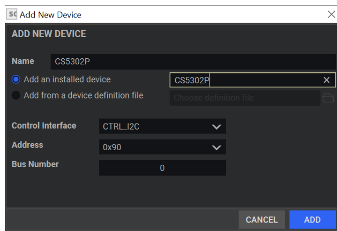
Figure 11: SoundClear Studio – Adding an Existing System
