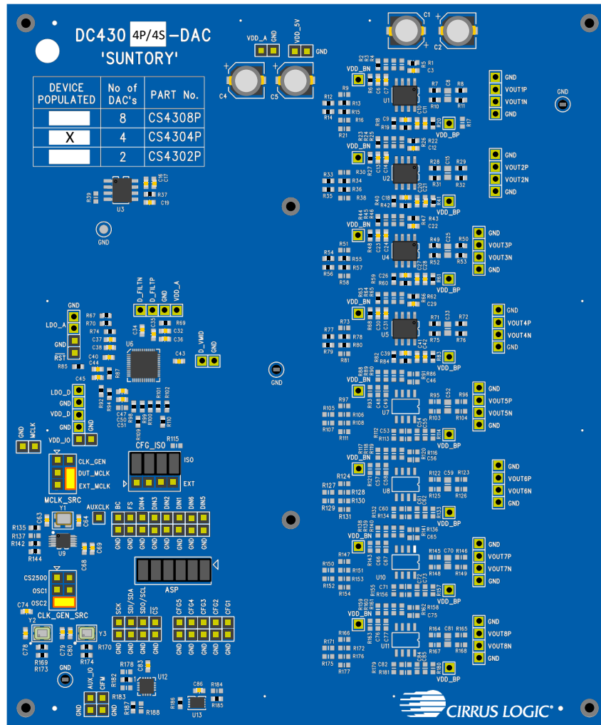
Figure 2: DC4304P/4S-DAC Daughter Card
