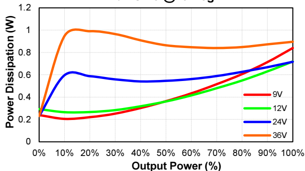
EC3SAW-24D05HP Pd Vs Po @25 Deg. C
