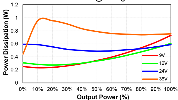
EC3SAW-24D12HP Pd Vs Po @25 Deg. C
