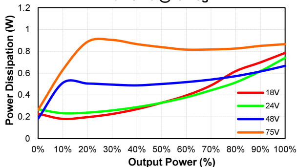
EC3SAW-48D05HP Pd Vs Po @25 Deg. C
