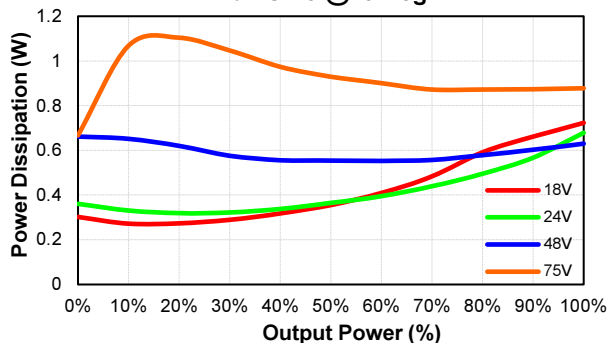
EC3SAW-48D15HP Pd Vs Po @25 Deg. C
