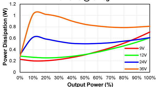
EC3SAW-24S12HP Pd Vs Po @25 Deg. C
