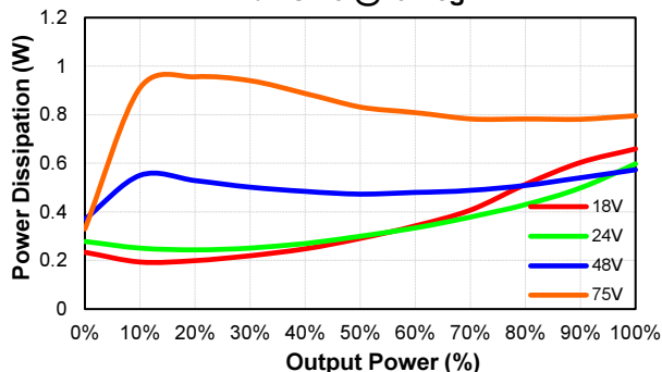
EC3SAW-48S15HP Pd Vs Po @25 Deg. C
