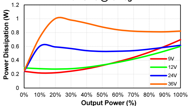
EC3SAW-24S15HP Pd Vs Po @25 Deg. C
