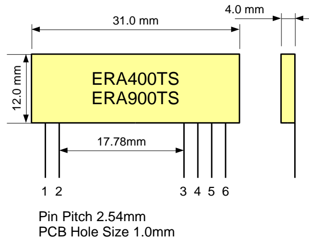
Physical Dimensions
