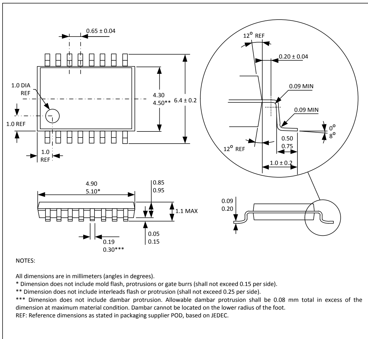
Figure 31 – TSSOP-16 Package Outline Dimensions
