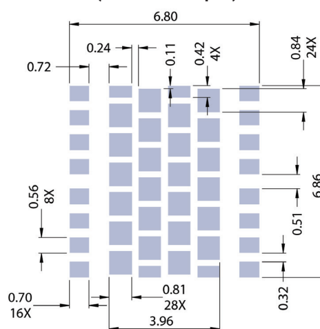
Recommended Stencil Openings 12 V Configurations (solid area is open)
