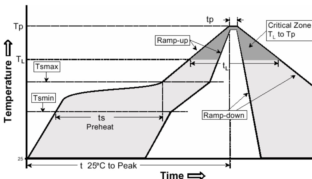
Figure 67: Reflow Condition
