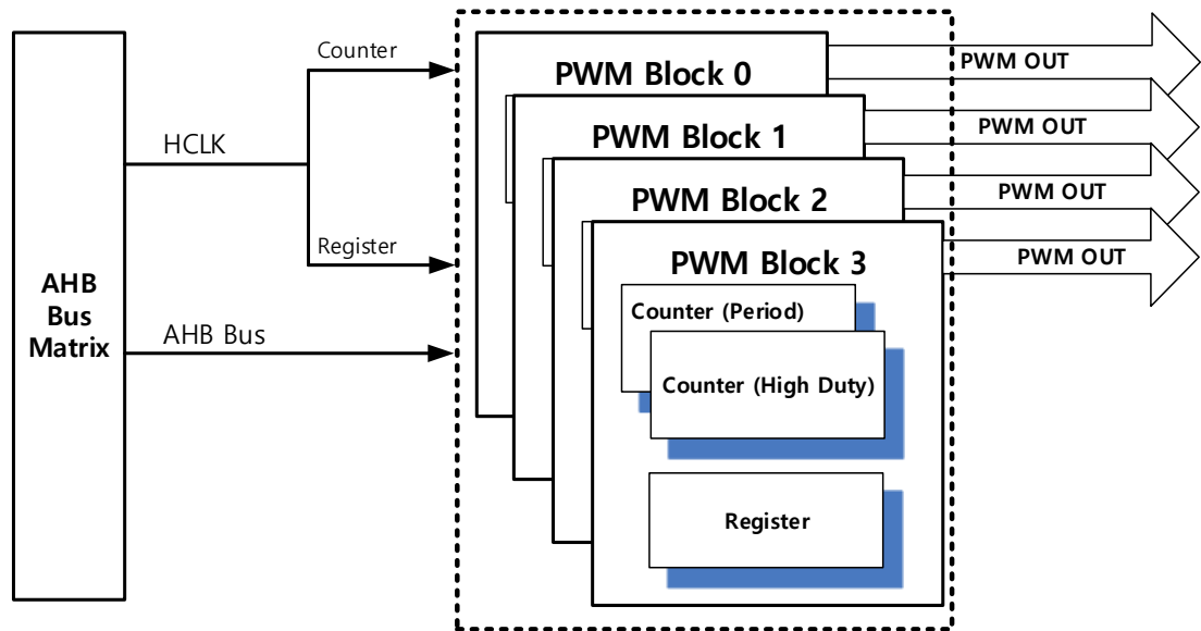
Figure 47: PWM Block Diagram
