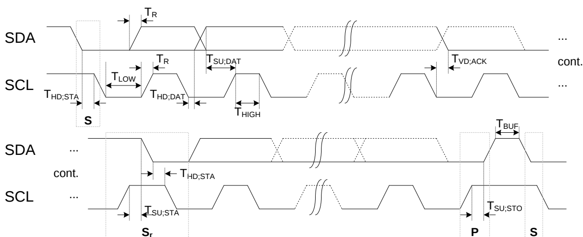
Figure 31: I2C Slave Timing Diagram
