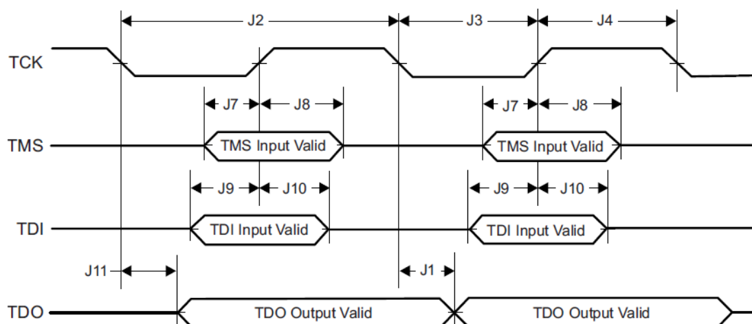
Figure 49: JTAG Timing Diagram
