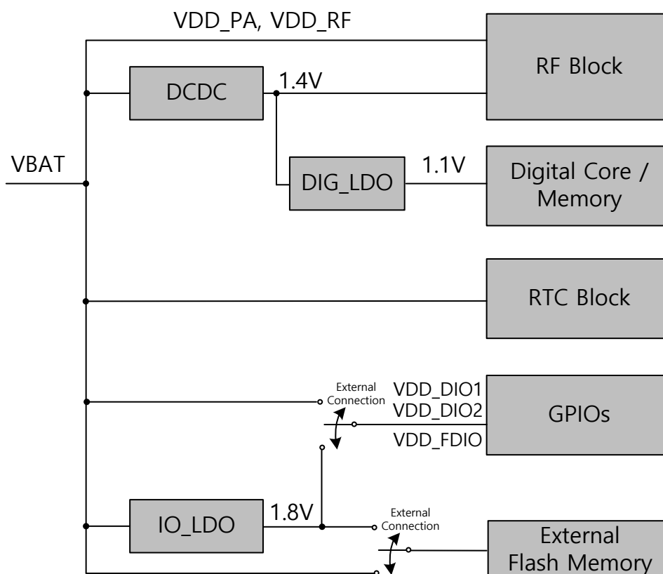
Figure 12: Power Management Block Diagram
