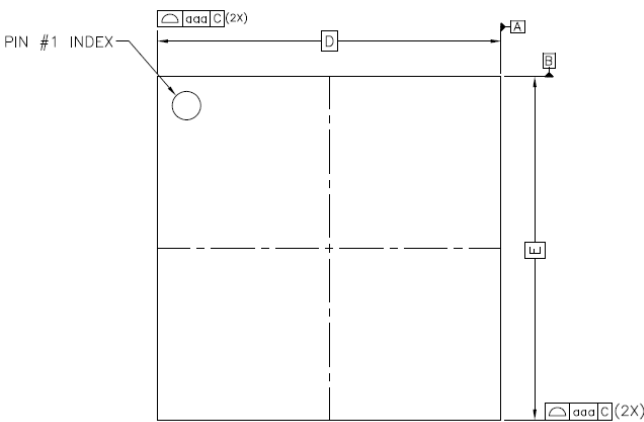
Figure 56: Top View
