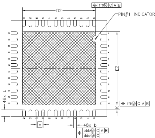
Figure 57: Bottom View
