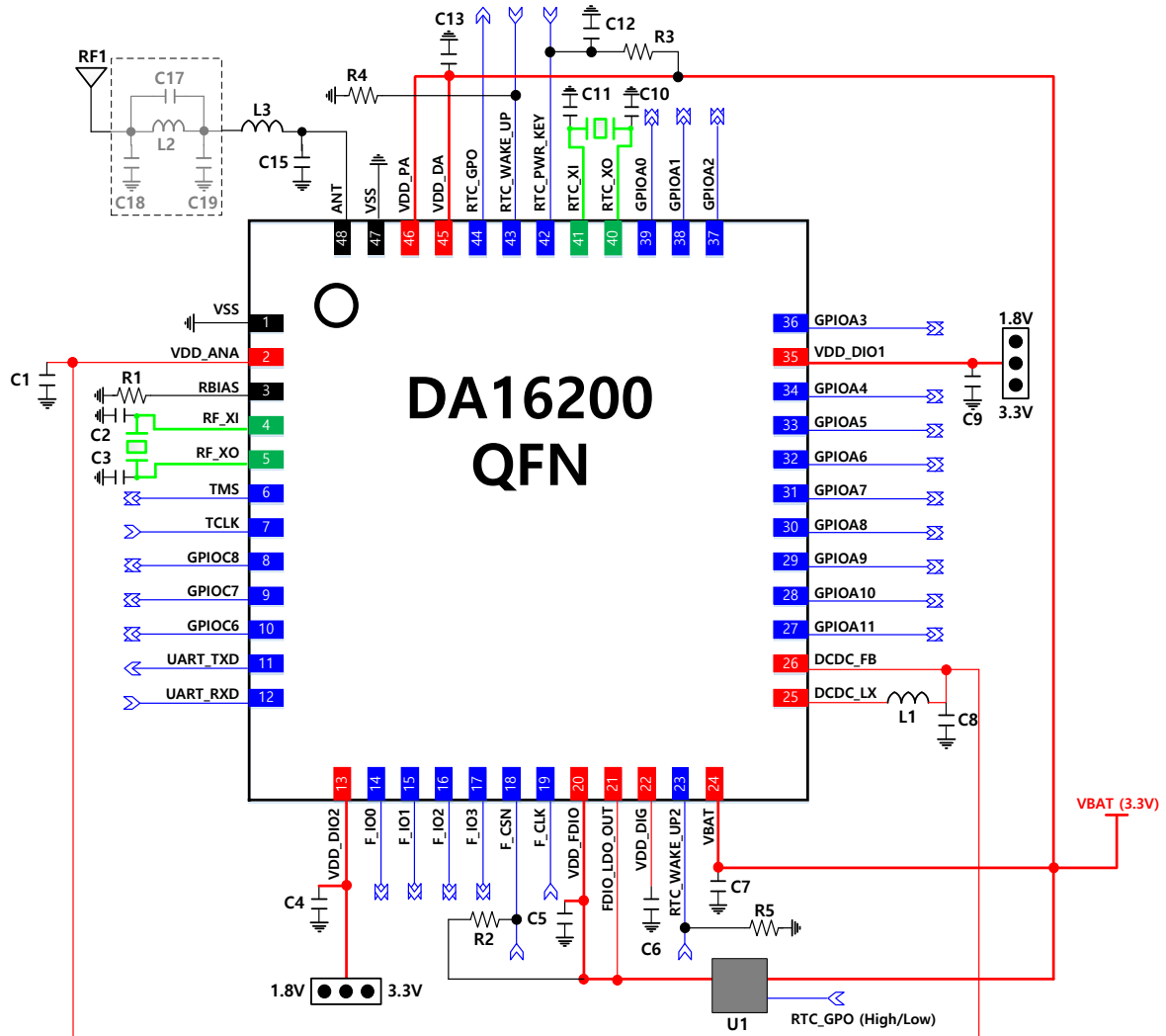
Figure 51: Typical Application – QFN, 3.3 V Flash
