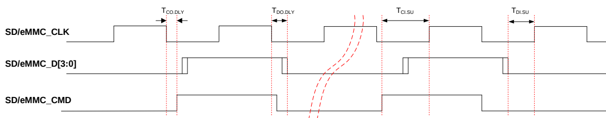
Figure 33: SD/eMMC Master Timing Diagram
