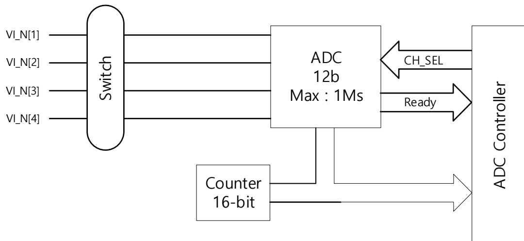
Figure 39: ADC Control Block Diagram
