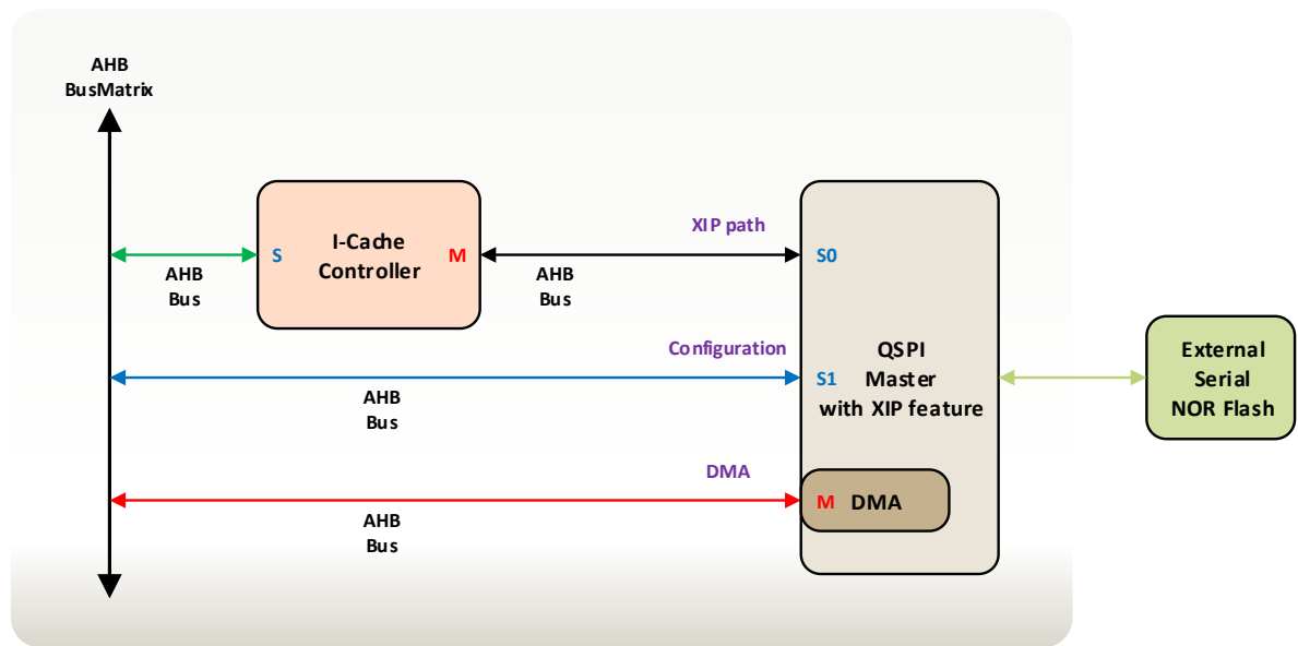
Figure 21: QSPI Master Block Diagram
