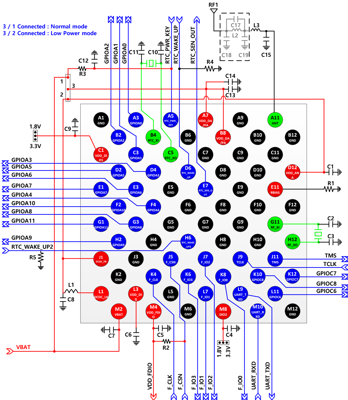
Figure 53: Typical Application – fcCSP, 1.8 V Flash
