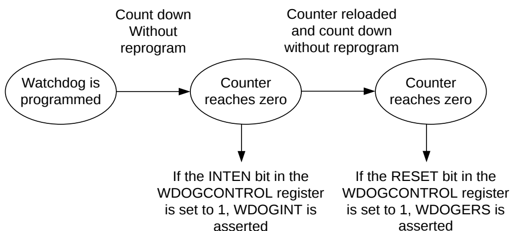
Figure 19: Watchdog Operation Flow Diagram
