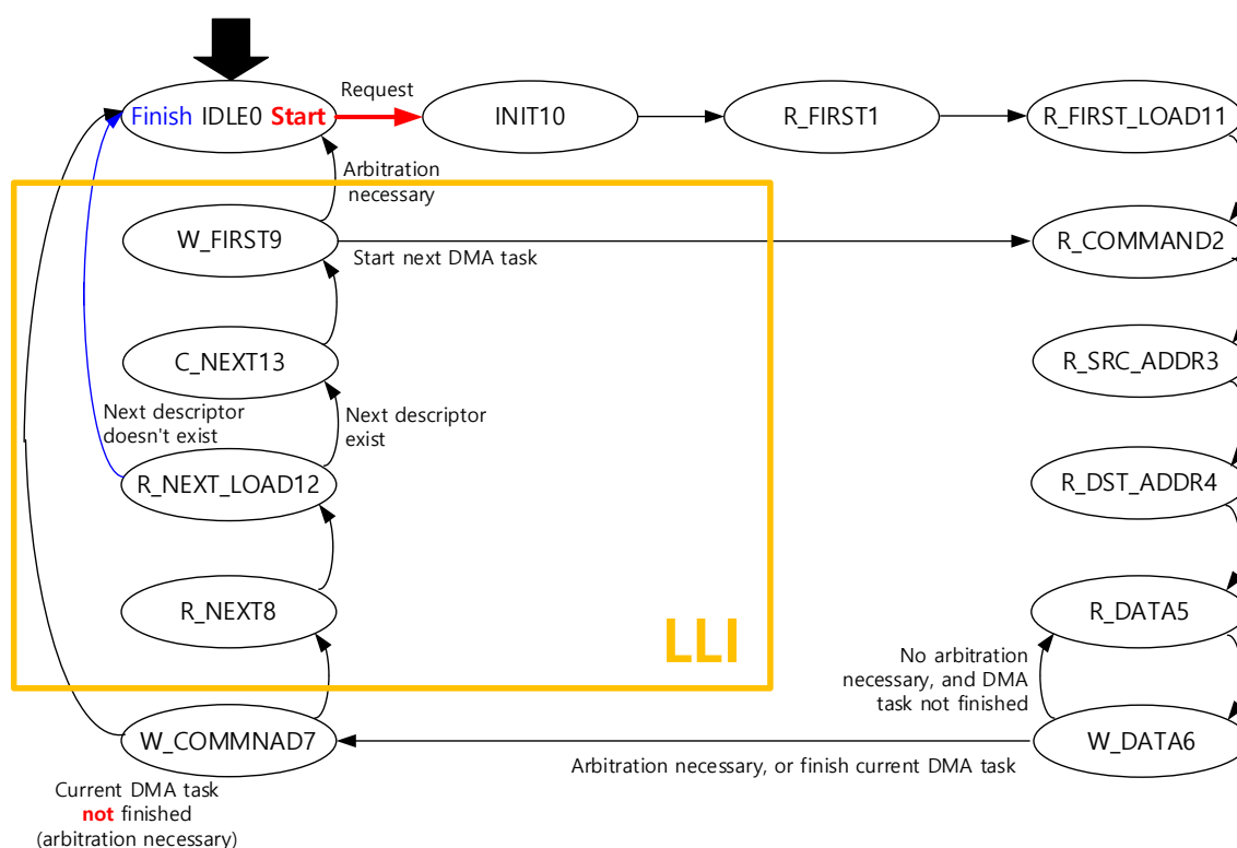
Figure 16: DMA1 State Machine
