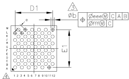
Figure 61: Bottom View
