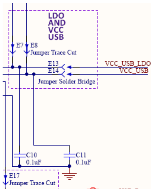
Figure 31. VCC_USB_LDO Circuit
