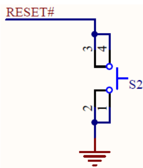
Figure 18. Reset Switch Circuit
