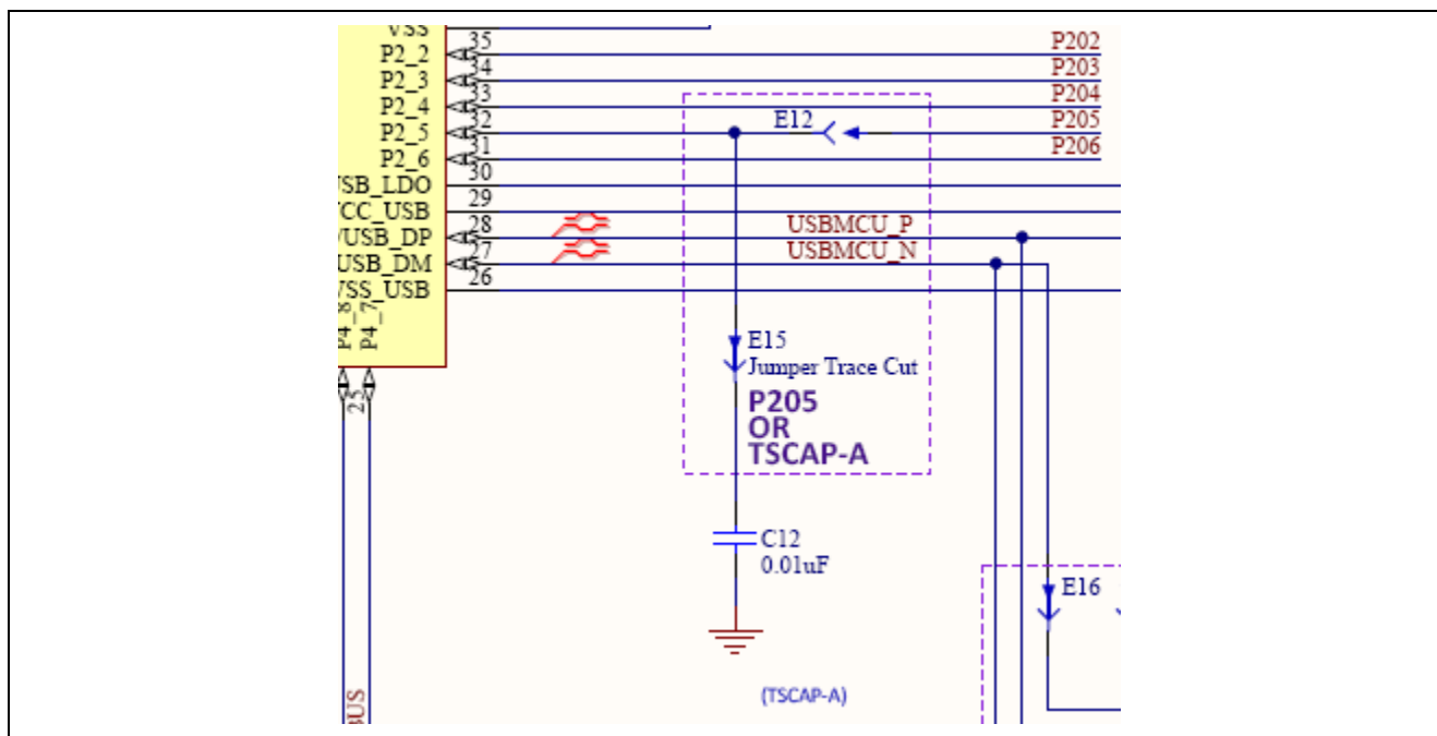
Figure 32. P205 Circuit
