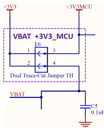
Figure 12. MCU Current Measurement Circuit
