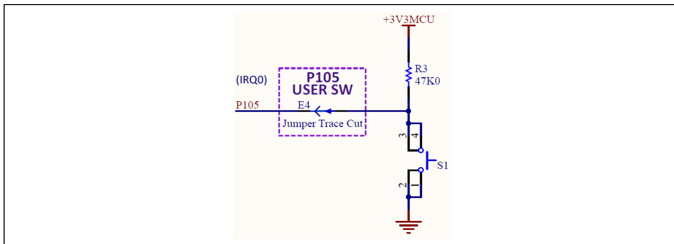
Figure 16. User Switch Circuit
