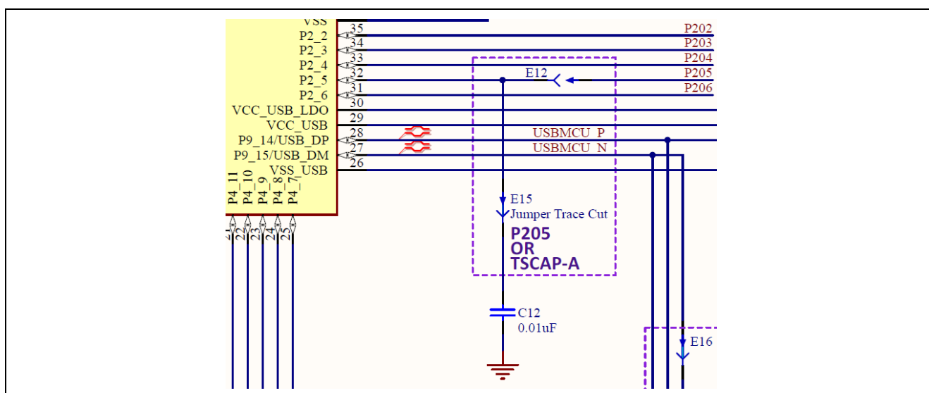
Figure 21. Capacitive Touch TSCAP Circuit
