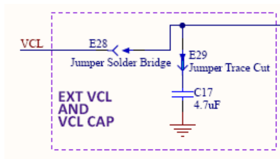
Figure 30. VCL and VCL Capacitor
