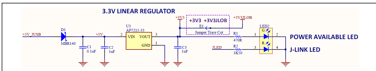
Figure 10. 3.3 V Power Regulator Circuit
