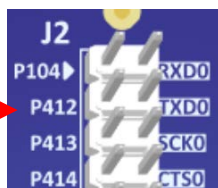
Figure 23. Fixed Function Pin Label Example
