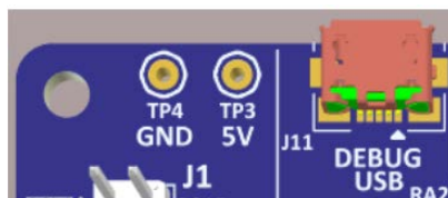
Figure 7. USB Debug Connector (J11), TP3, and TP4 on the Evaluation Kit Board
