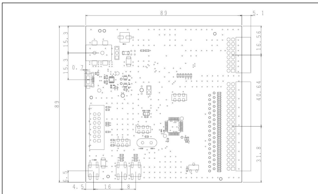
Figure 2-3. Board Dimensions
