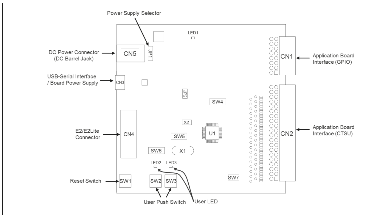
Figure 2-2. Parts Location
