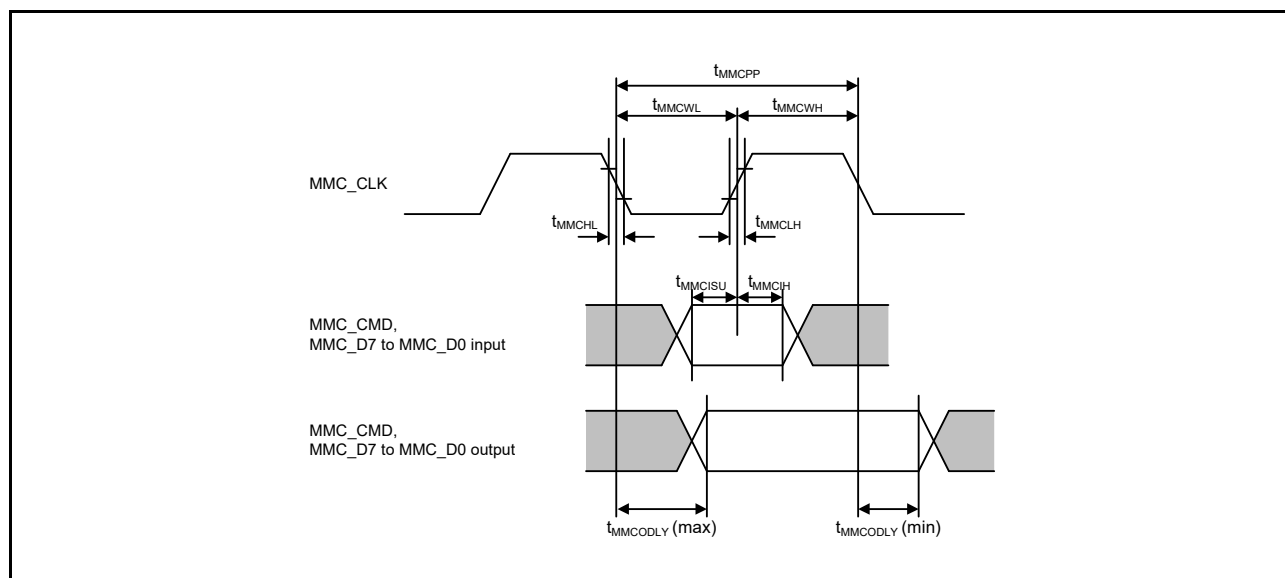
Figure 2.74 MMC Interface
