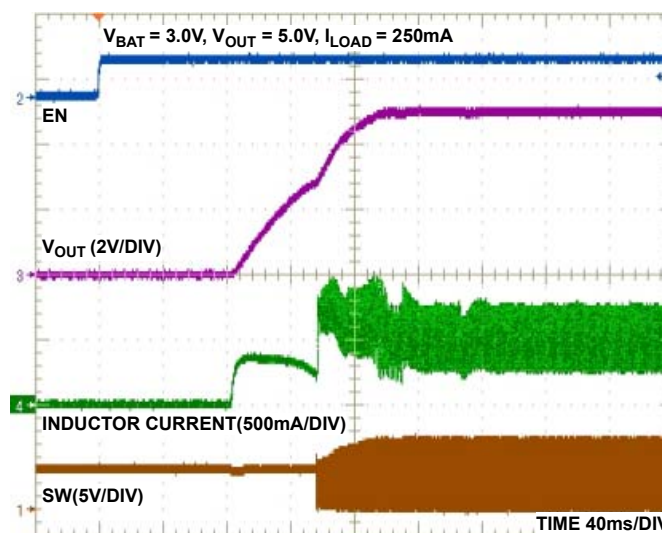
FIGURE 11. START-UP AFTER ENABLE ( I_{LOAD} = 250mA )
