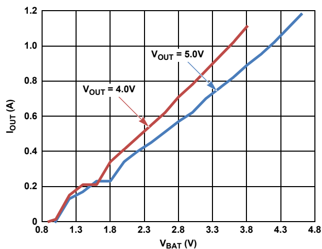
FIGURE 7. MAXIMUM OUTPUT CURRENT vs INPUT VOLTAGE (ISL9113ERAZ)
