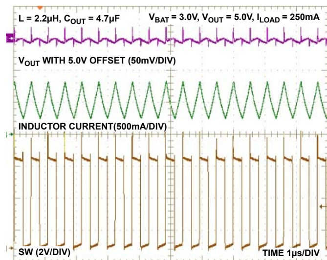
FIGURE 10. PWM WAVEFORM
