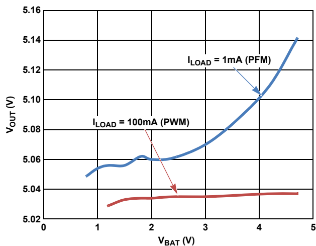
FIGURE 8. LINE REGULATION, V_{OUT} = 5V (ISL9113ER7Z)
