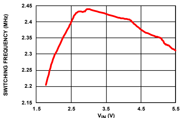
FIGURE 7. SWITCHING FREQUENCY vs INPUT VOLTAGE
