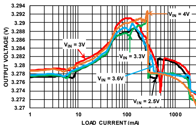
FIGURE 5. OUTPUT VOLTAGE vs LOAD CURRENT
