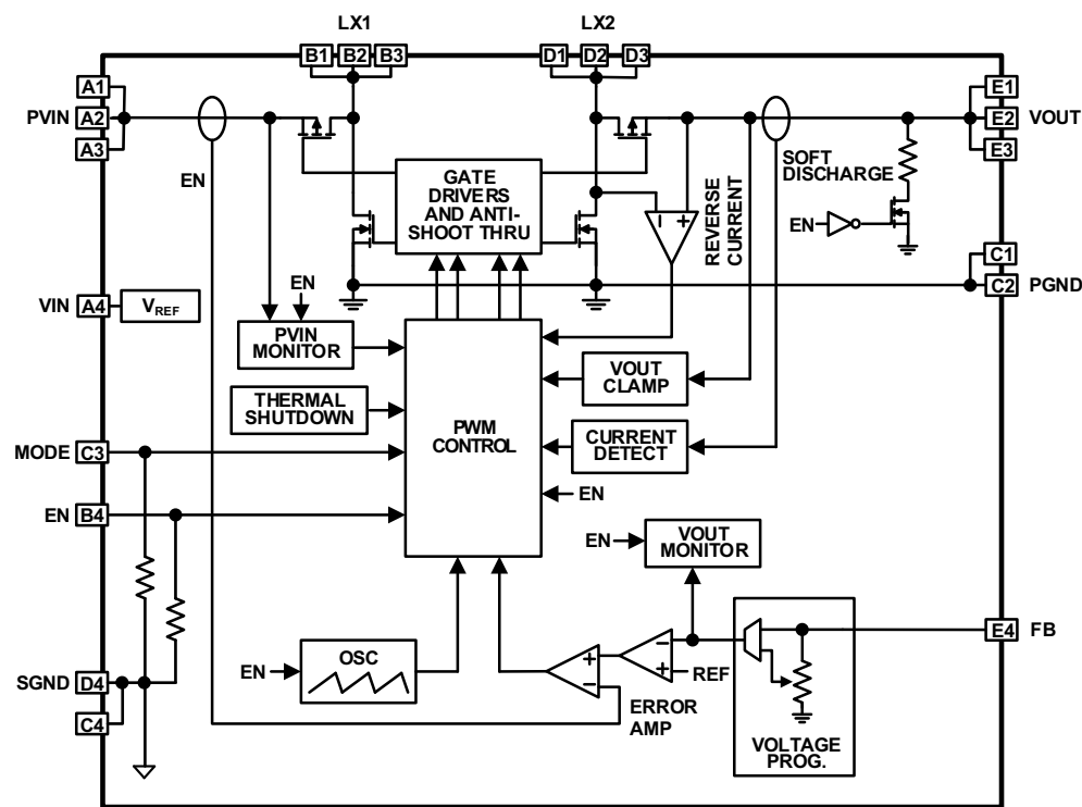
FIGURE 3. BLOCK DIAGRAM
