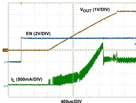
FIGURE 11. SOFT-START ( V_{IN} = 3.6\text{V} , V_{OUT} = 3.3\text{V} , 1A LOAD)
